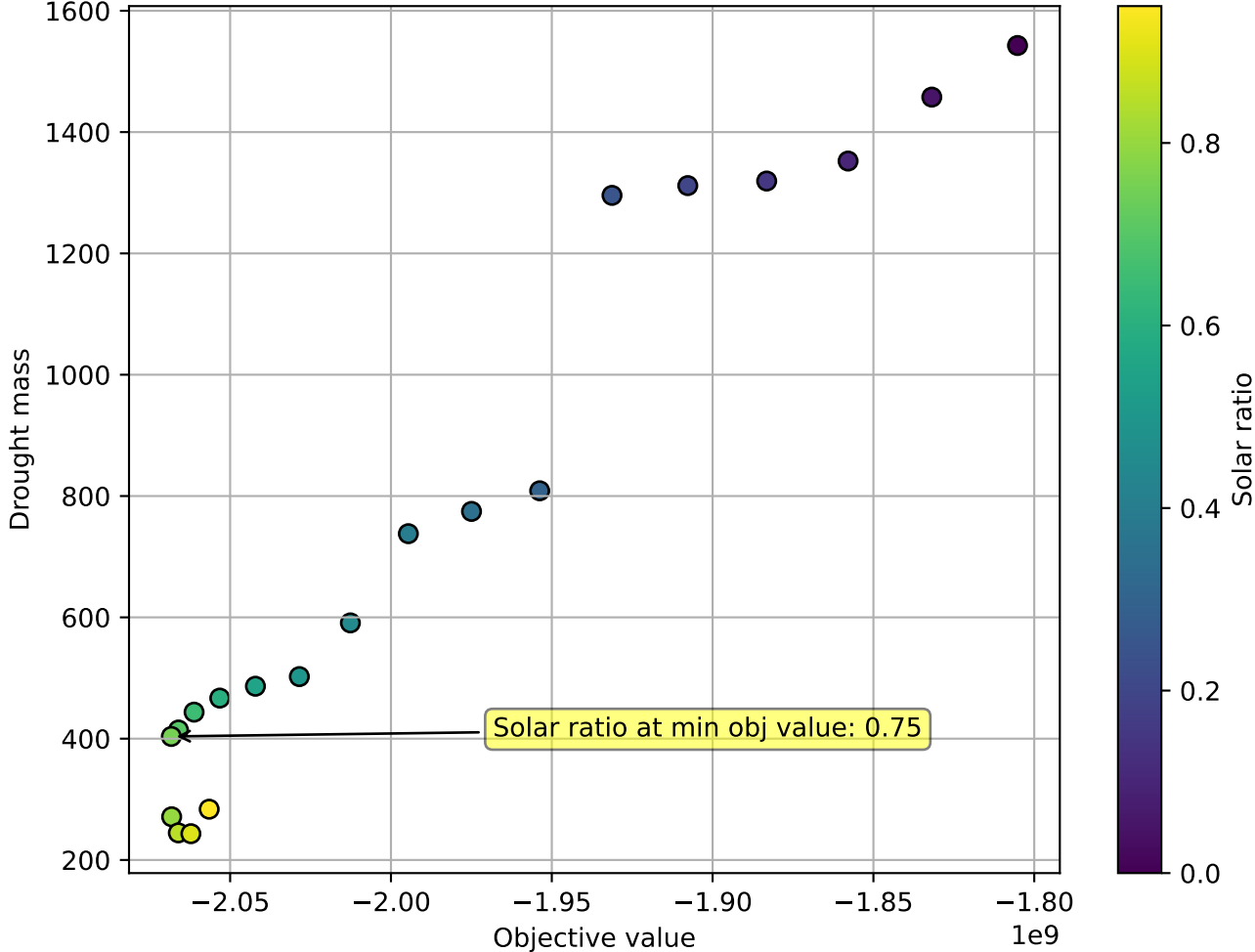
Objective value vs drought mass, with respect to solar ratio (1.3 Dunkleflaute)
