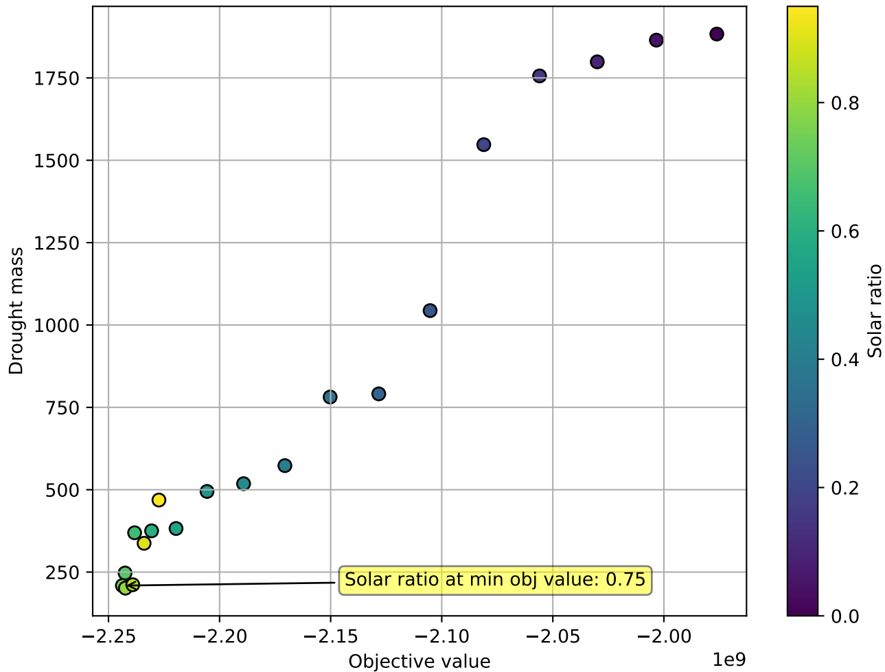
Objective value vs drought mass, with respect to solar ratio (1.5 Dunkleflaute)
