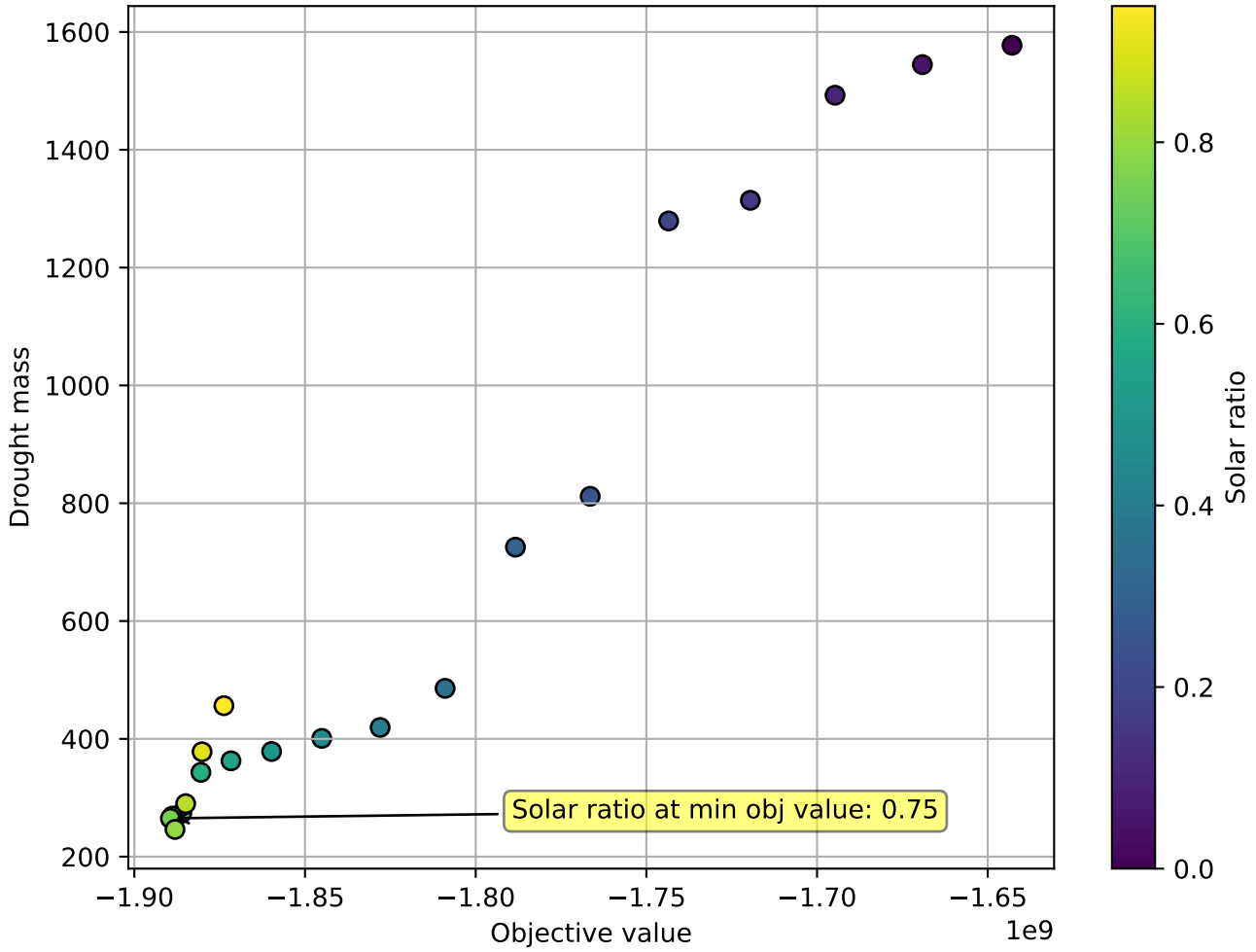
Objective value vs drought mass, with respect to solar ratio (1.7 Dunkleflaute)
