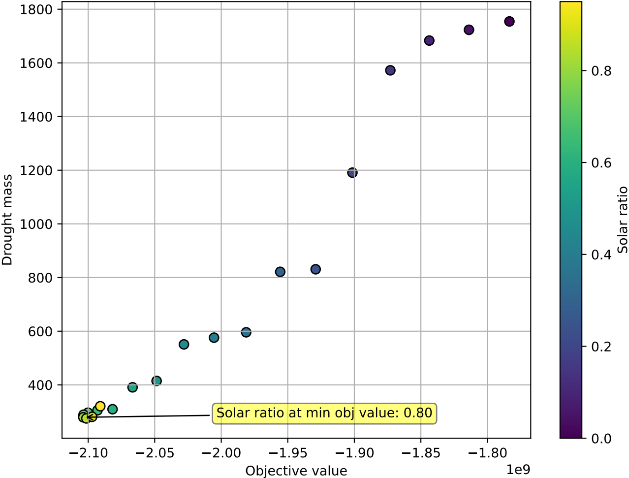
Objective value vs drought mass, with respect to solar ratio (2.0 Dunkleflaute)
