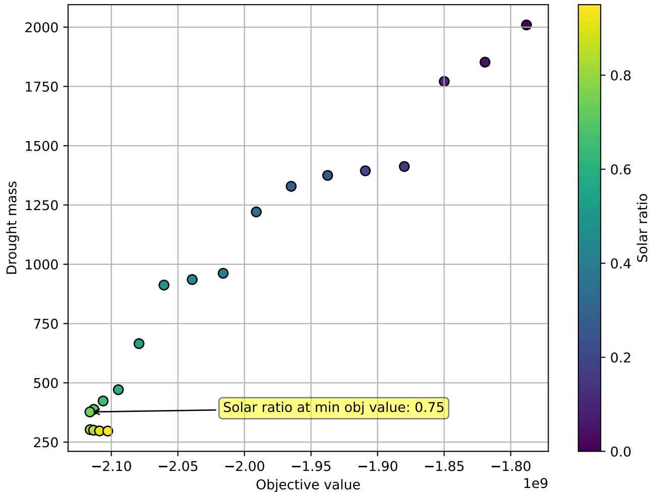
Objective value vs drought mass, with respect to solar ratio (3.0 Dunkleflaute)
