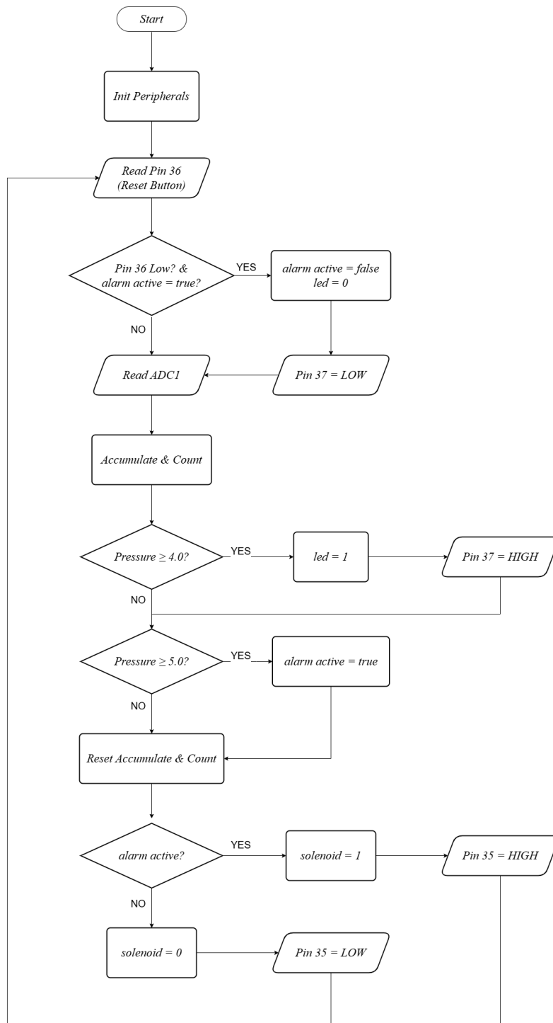
Figure 2: MS-LSIS algorithm flowchart with two stages ( warning and trip ) and the latching mechanism.
