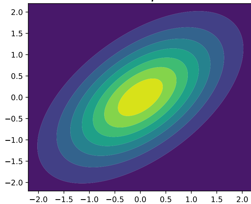
\varepsilon = 2 and \rho = 0.95
