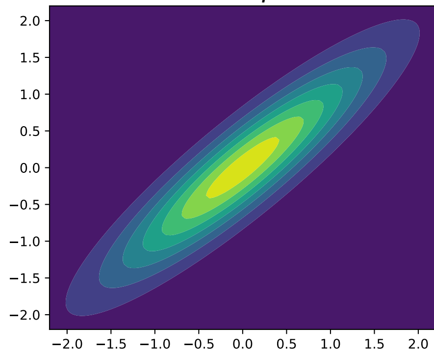
\varepsilon = 2 and \rho = 0.9
