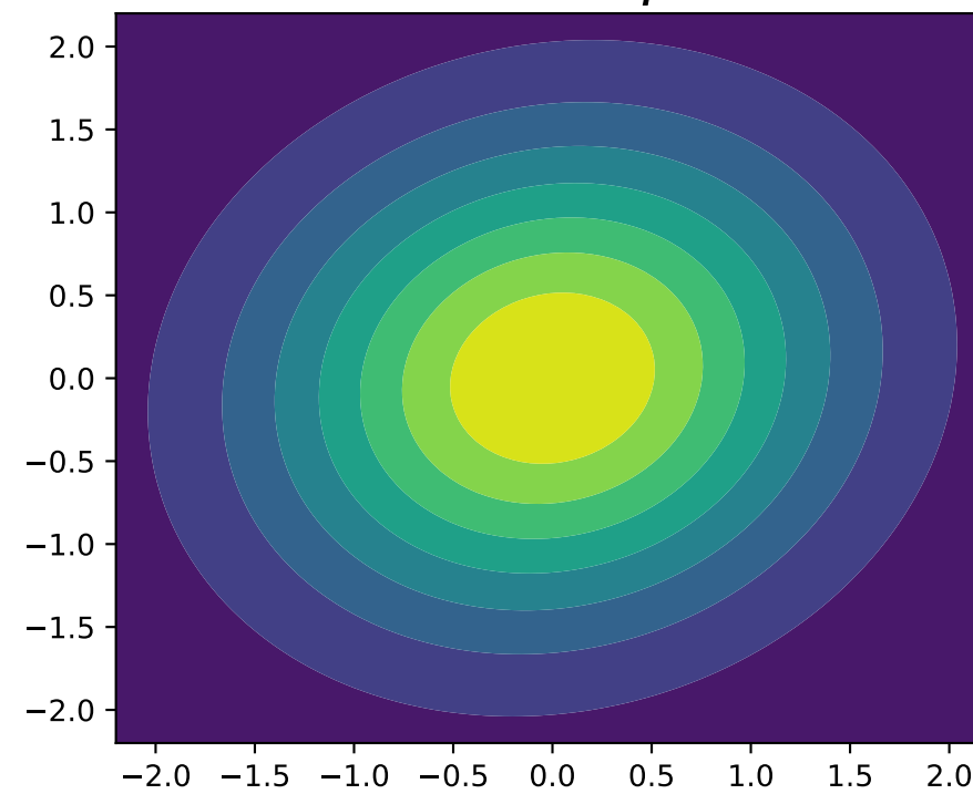
\varepsilon = 10 and \rho = 0
