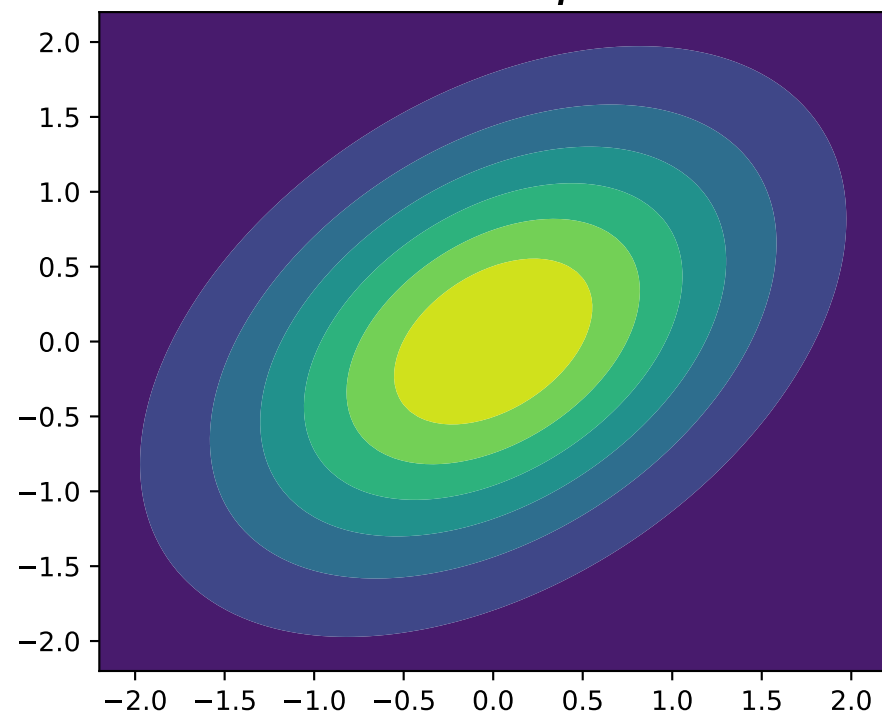
\varepsilon = 2 and \rho = 0
