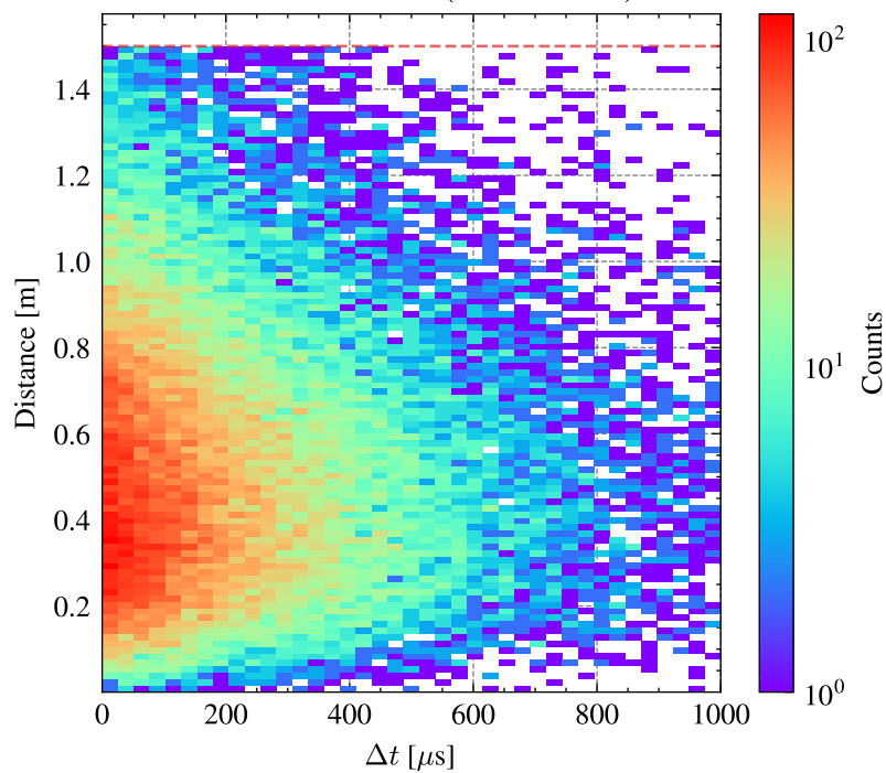
Time vs Distance (RUN10110)
