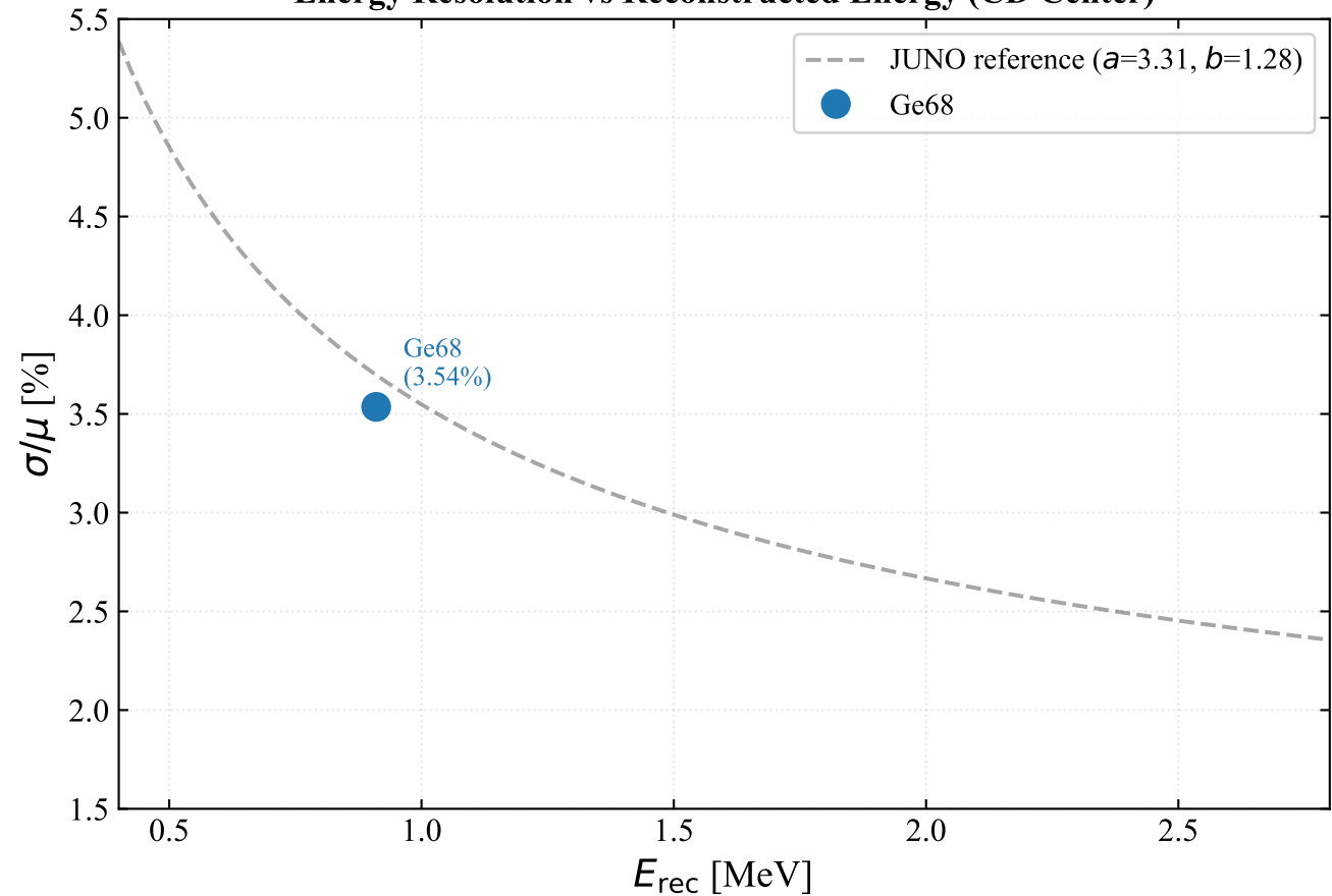
Energy Resolution vs Reconstructed Energy (CD Center)
