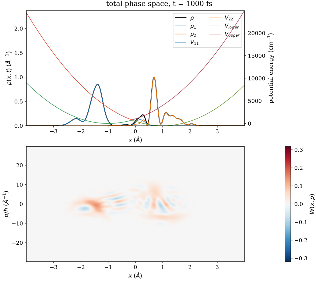
Figure 4: Coordinate-space and phase-space view of the product-damped trajectory at 1.0 ps. The upper panel overlays total and diabatic densities on the diabatic and adiabatic potential surfaces. The lower panel shows the electronic-state-traced nuclear Wigner function versus x and p/\hbar . Positive and negative lobes resolve counterpropagating structure and coherent interference hidden by |\psi(x)|^2 . This single-trajectory quasiprobability is diagnostic rather than a mechanism label; stochastic ensemble claims require averaging consistently sampled trajectories.
