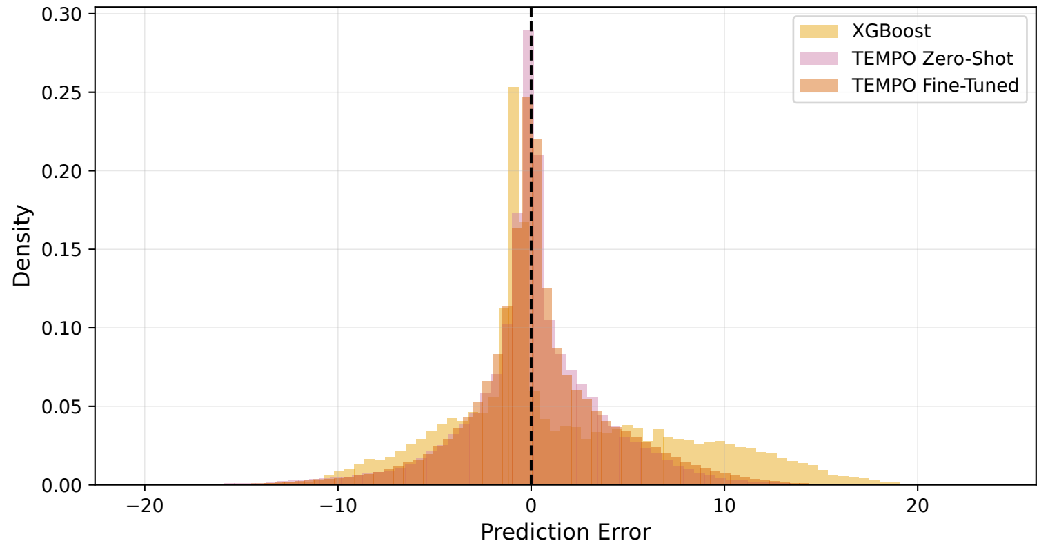
SE-Htm (Forest)
