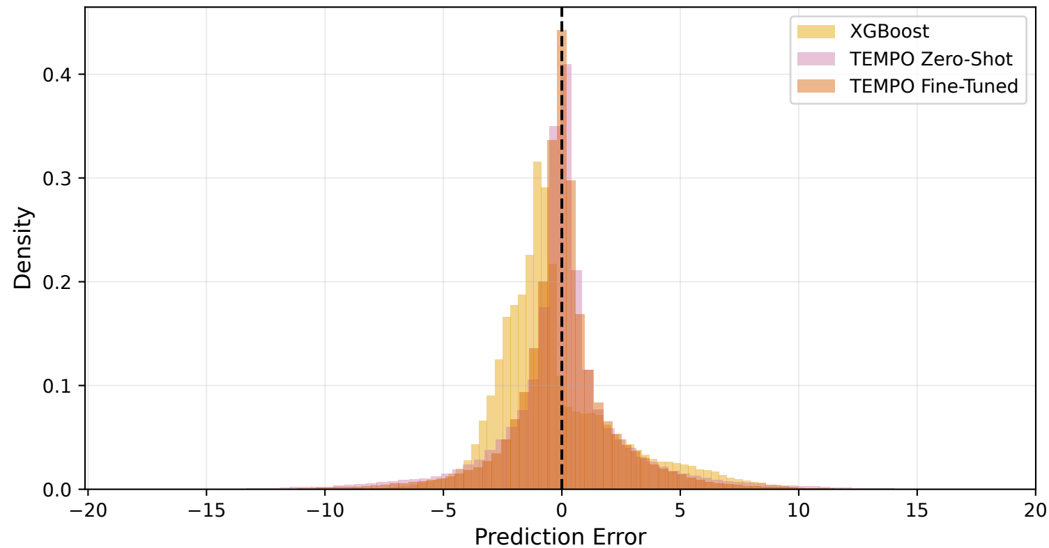
UK-AMo (Wetland)
