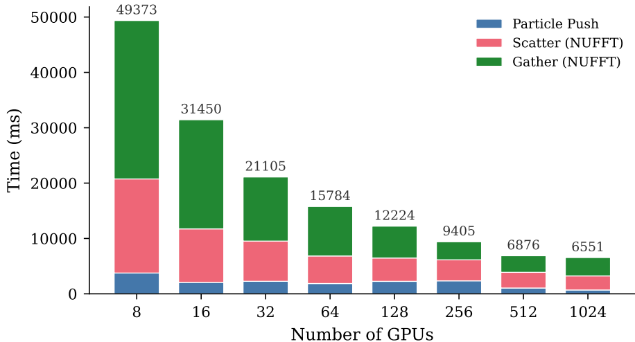
Component Breakdown (Pruned)
