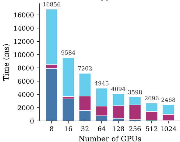
Scatter (Type-1 NUFFT)
