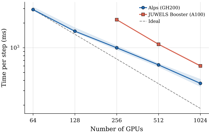
PIF Grid 1024^3 (full FFT, \varepsilon = 10^{-4} )
