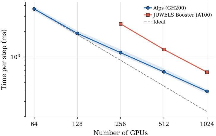
PIF Grid 1024^3 (full FFT, \varepsilon = 10^{-8} )
