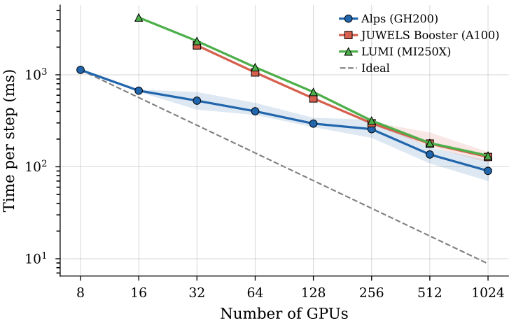
PIF Grid 512^3 (full FFT, \varepsilon = 10^{-4} )
