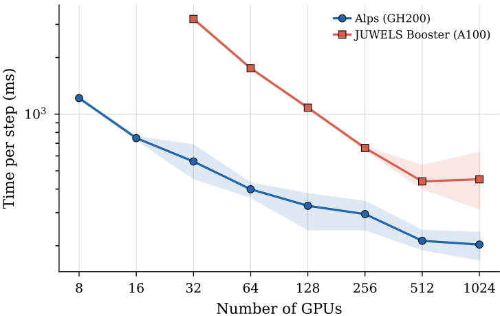
PIF Grid 512^3 (pruned FFT, \varepsilon = 10^{-4} )
