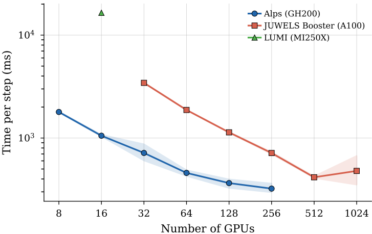
PIF Grid 512^3 (pruned FFT, \varepsilon = 10^{-8} )
