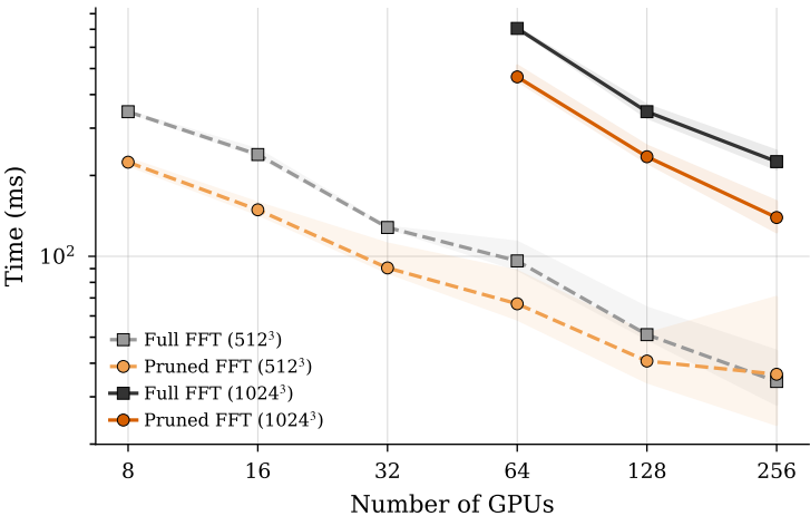
Forward FFT — Concurrency 4 (Alps)
