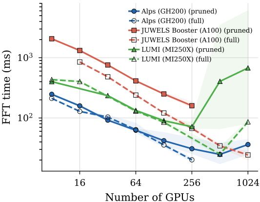
Grid 512 3
