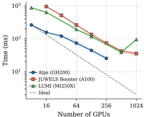
Type-2 (interpolation)
