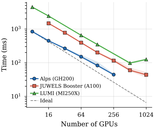
Type-1 (spreading)
