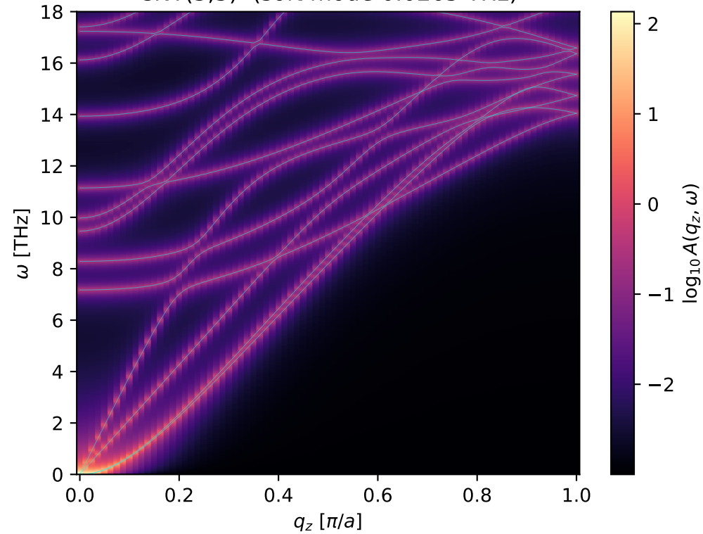
CNT(3,3) (soft mode 0.0265 THz)
