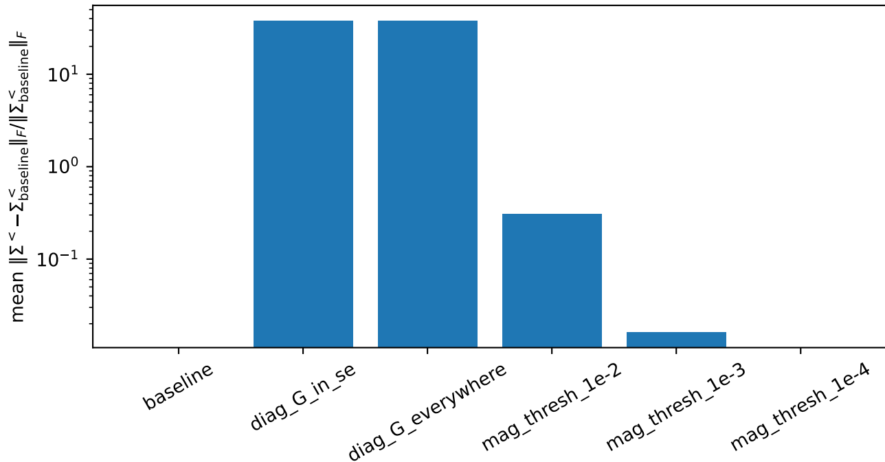
Cutoff sensitivity of phonon-phonon SSE
