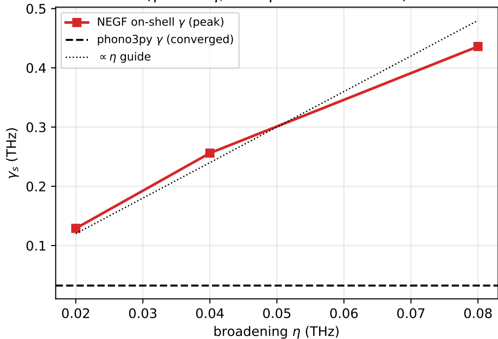
On-shell peak ratio is a broadening artifact ( \gamma^{NEGF} \propto \eta ; the spurious 'factor 4')
