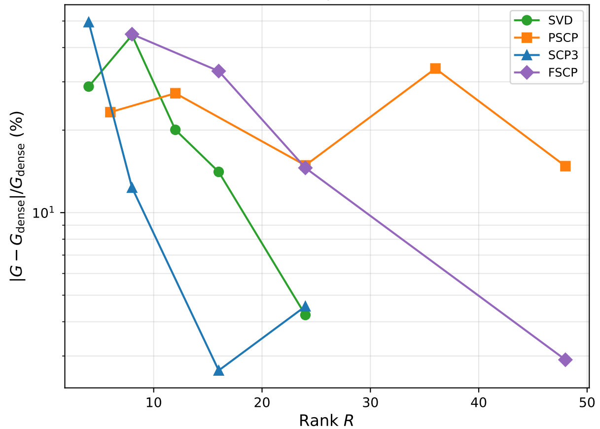
(b) Relative transport error vs rank
