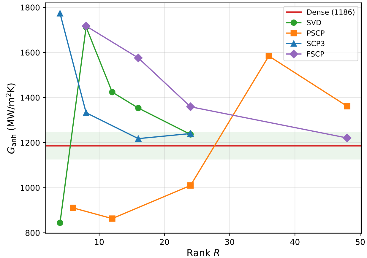
(a) Thermal conductance vs rank
