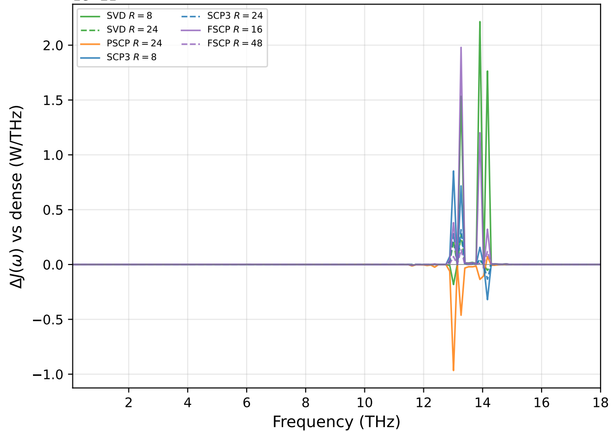
1e-21 (b) Spectral current difference
