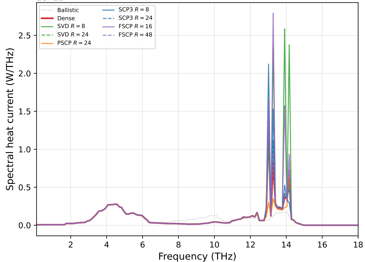
1e-21 (a) Spectral heat current
