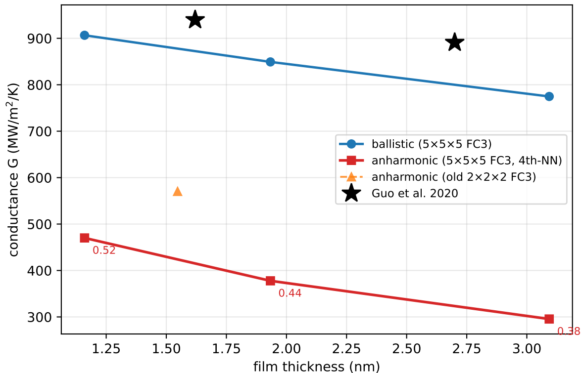
Cross-plane Si thin film: high-quality 5×5×5 FC3 (native prefactor; G_{anh}/G_{ball} annotated)
