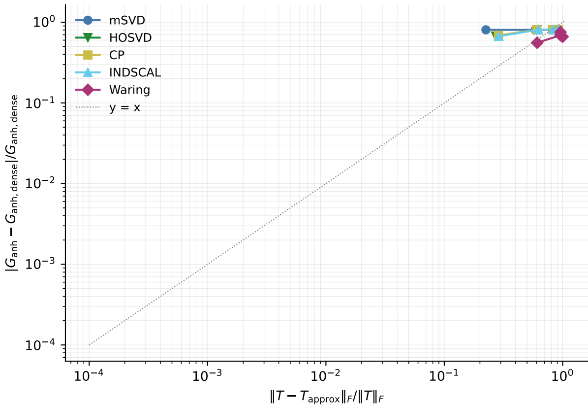
Predictive value of Frobenius error for thermal-conductance error
