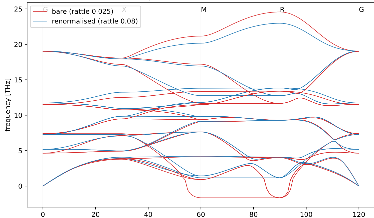
SrTiO 3 : rattle amplitude renormalises the soft mode (= SCP)
