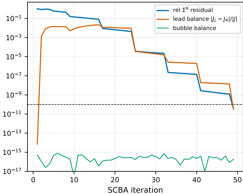
convergence measure
