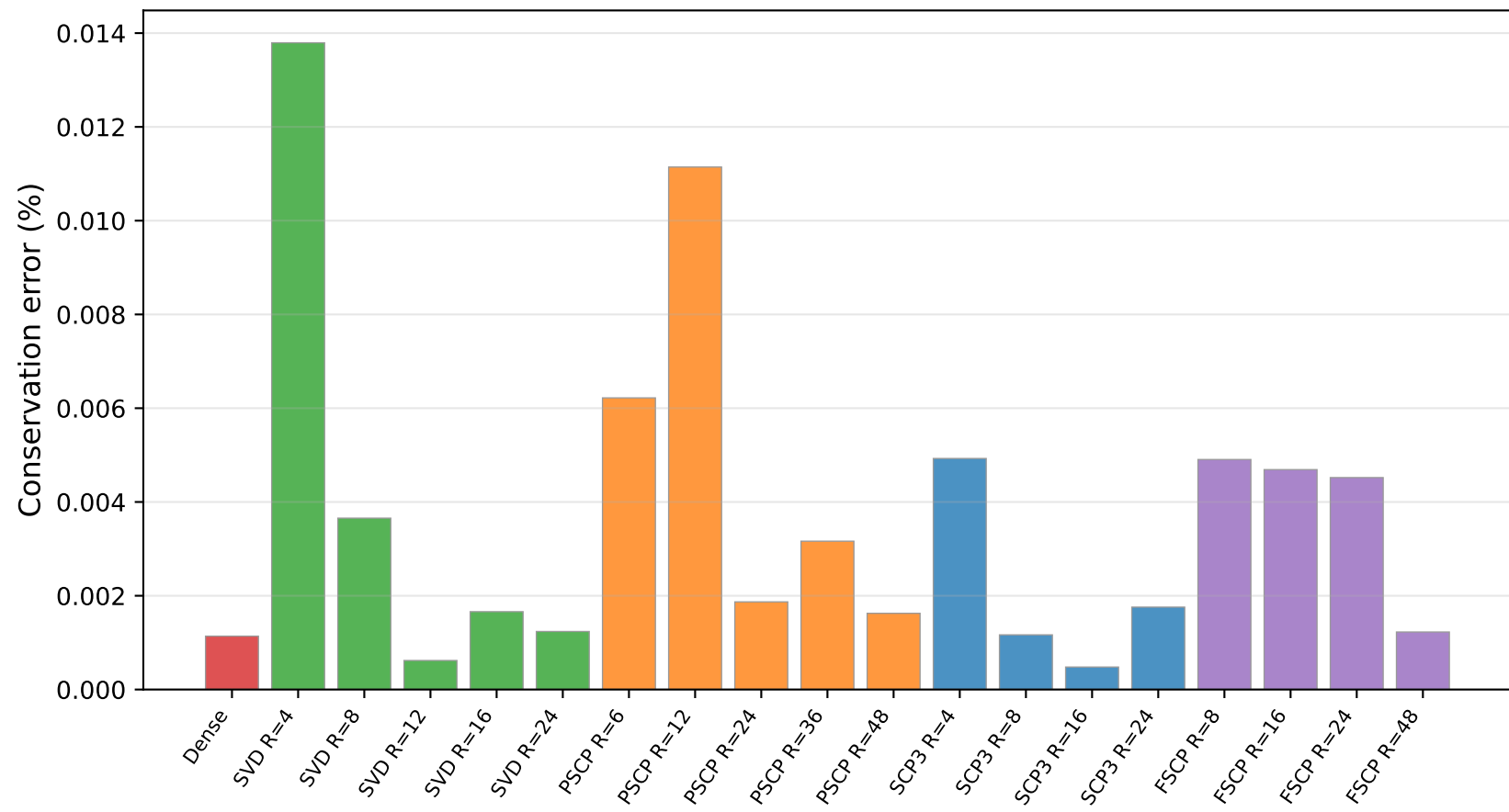
Heat flow conservation error
