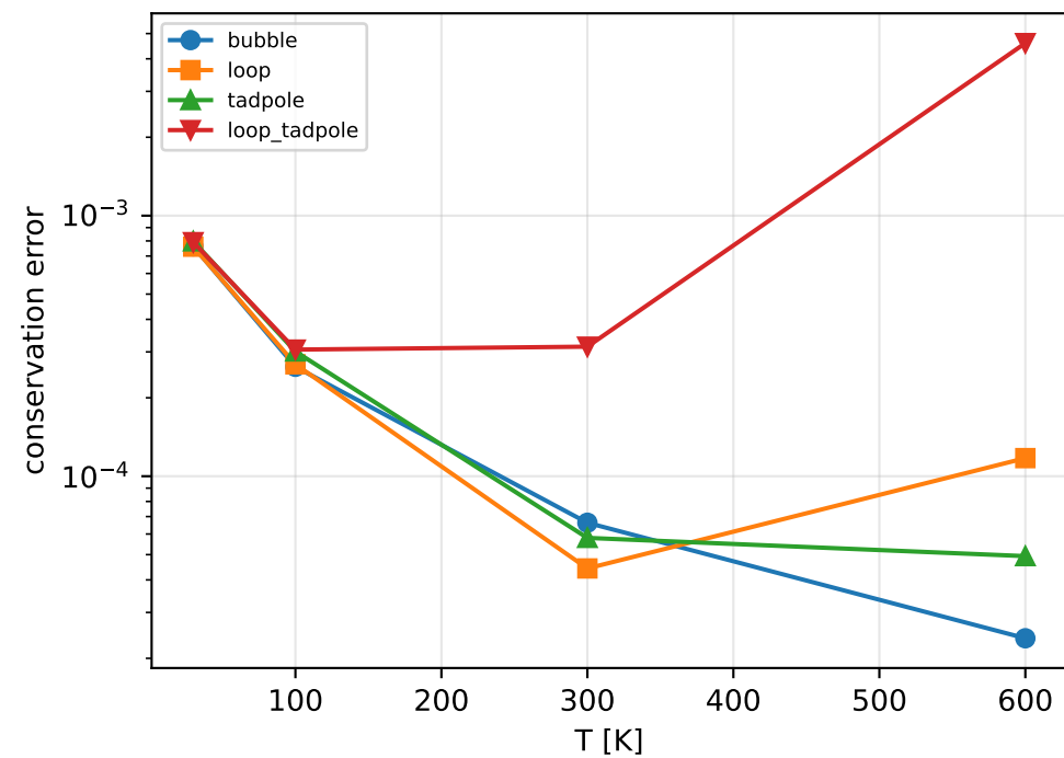
cnt33: heat-flow conservation vs mode
