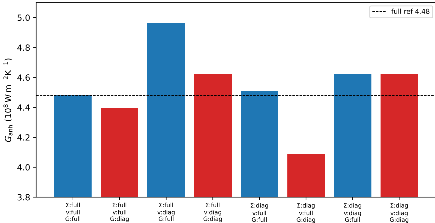
(3,3) cutoff hierarchy (n_slabs=2): robust ( \pm 10\% ); red = diagonal-G
