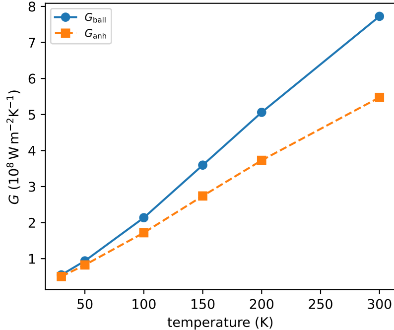
(3,3) conductance vs T (L=1)
