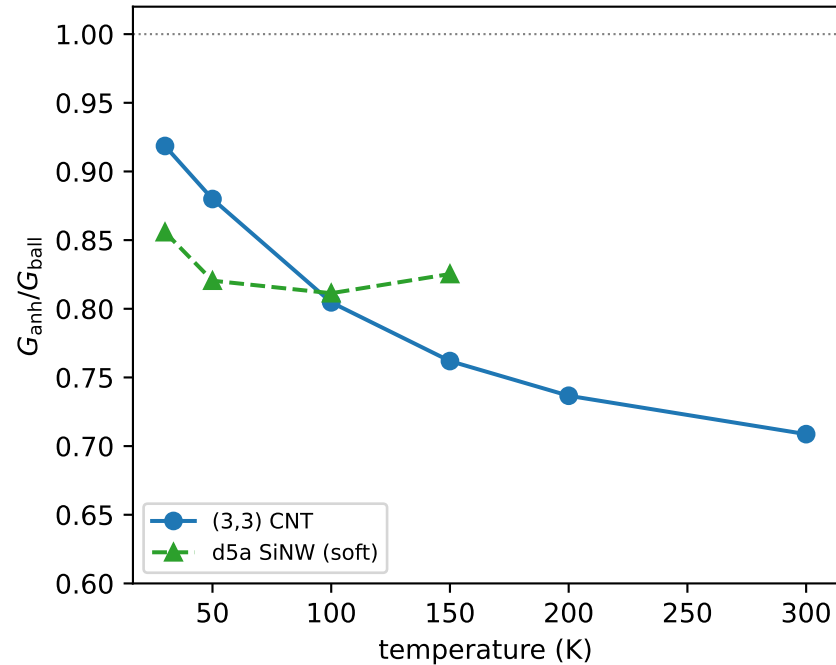
Channel freezing: \rightarrow 1 as T \rightarrow 0
