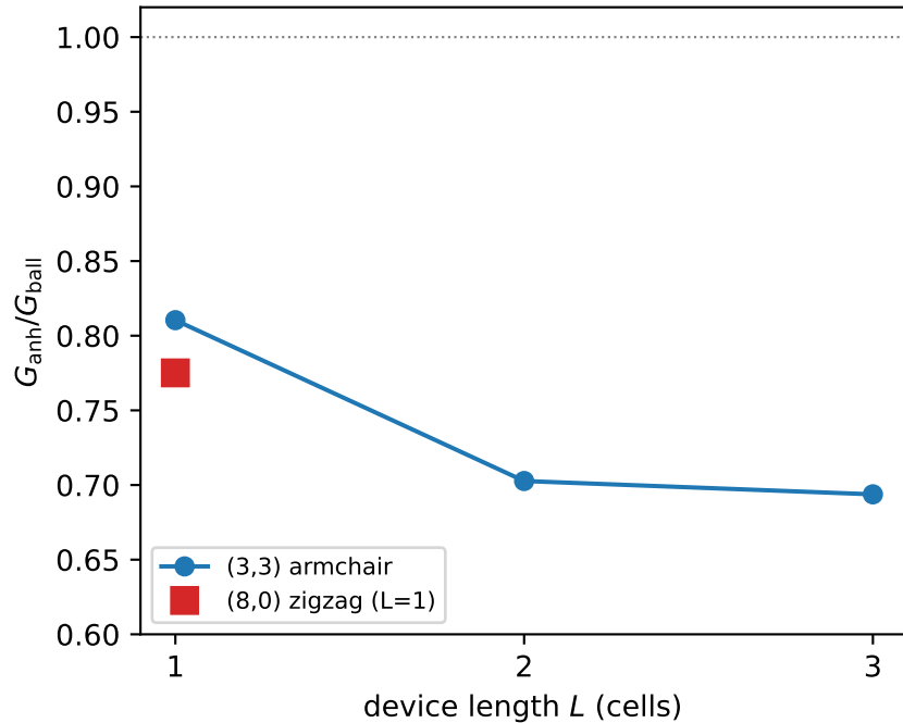
Length ladder (300 K)
