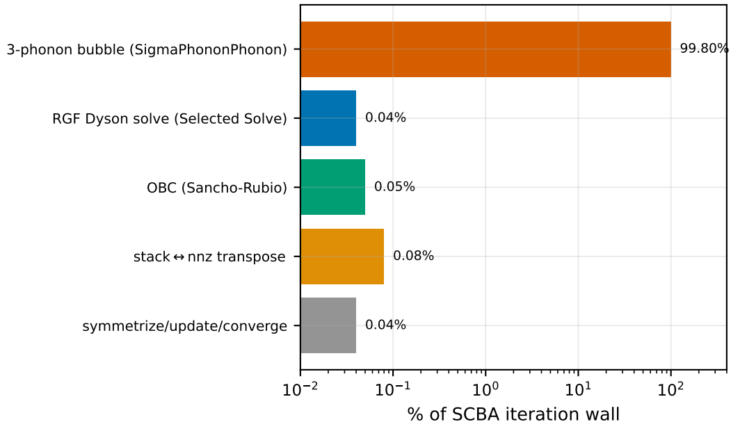
Per-phase profile (CNT L = 4 , single rank)
