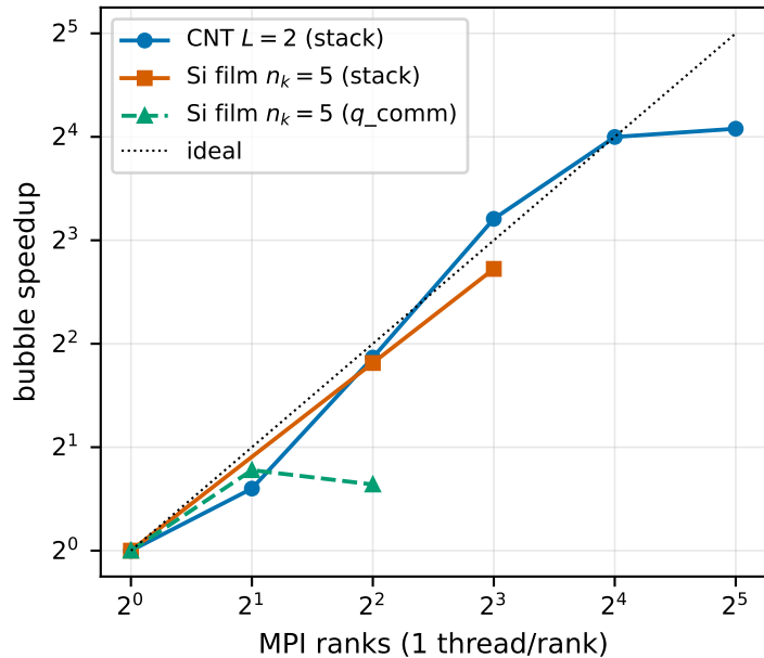
Strong scaling of the 3-phonon bubble
