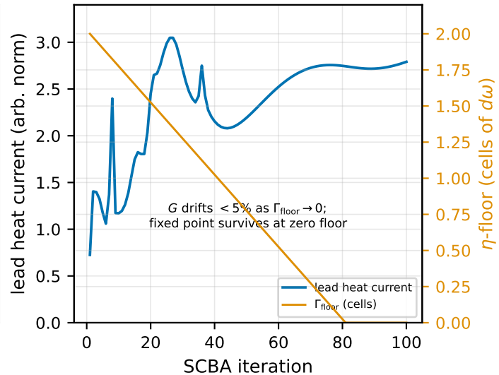
(c) floor anneal 2 \rightarrow 0
