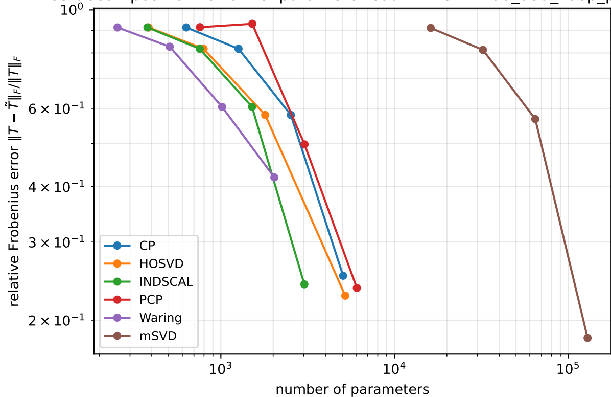
FC3 decomposition: error vs. parameter count — sinw100_d5a_vasp_ph
