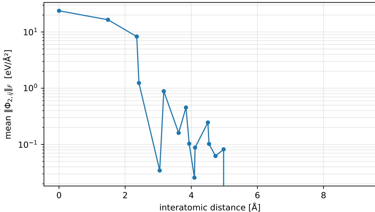
FC2 magnitude vs distance — sinw100_d5a_vasp_phonon
