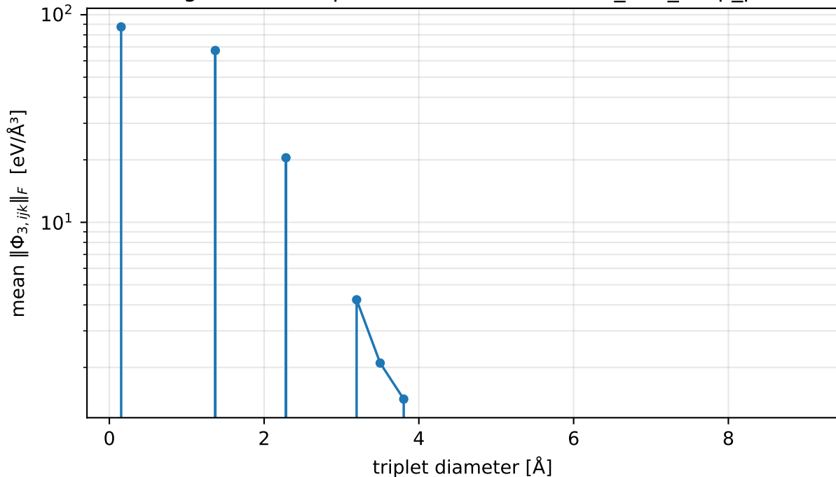
FC3 magnitude vs triplet diameter — sinw100_d5a_vasp_phonon
