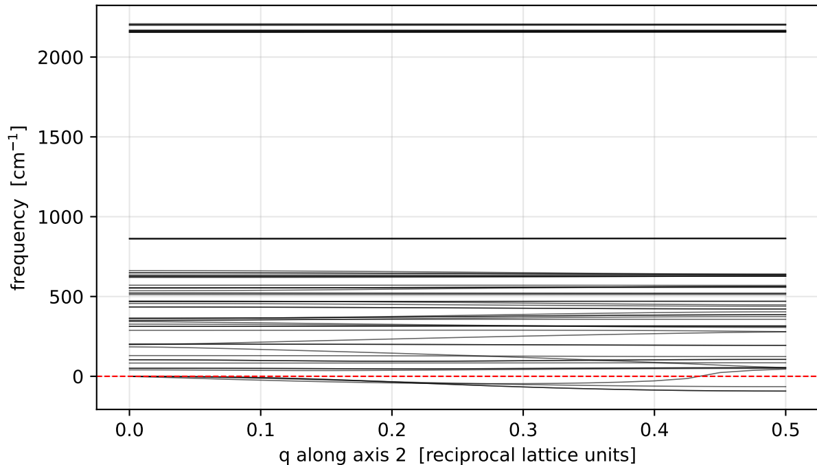
Phonon dispersion (sanity) — sinw100_d5a_vasp_phonon
