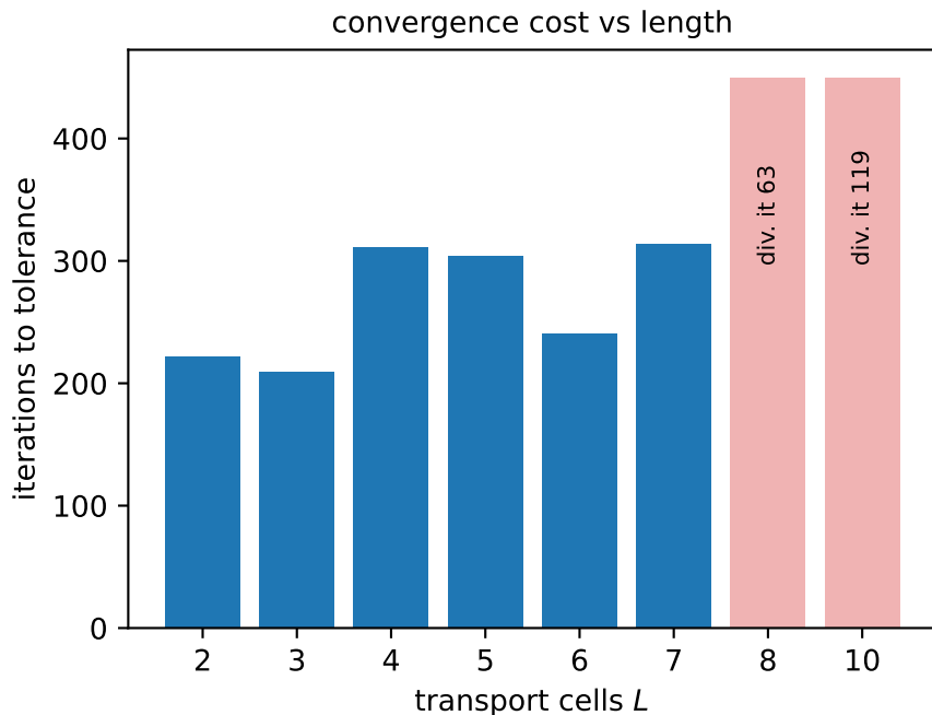
CNT(3,3), 300 K, exact bubble kernel (sse_g_band = 2): length series
