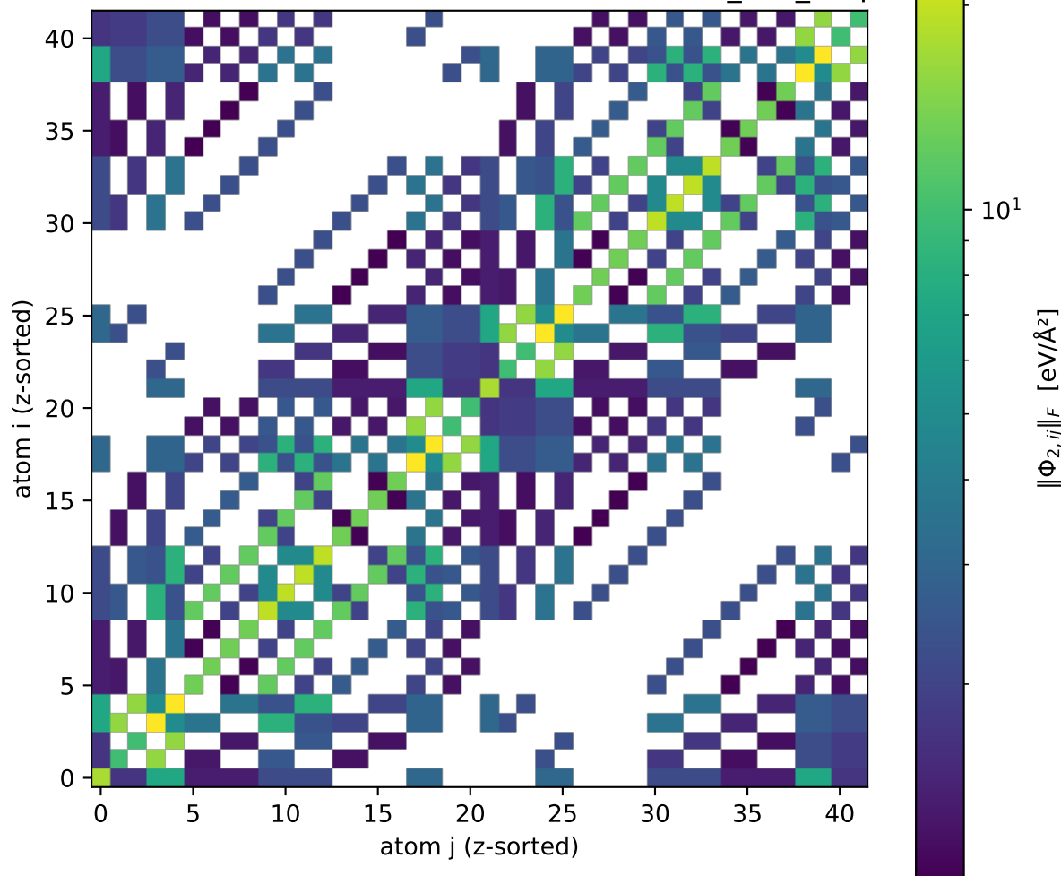
FC2 atomic-block Frobenius norm — sinw100_d5a_vasp
