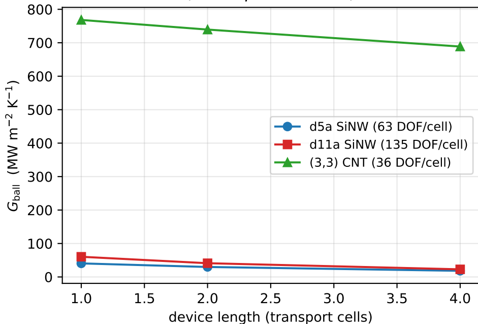
Coherent conductance vs length at T = 300 K (finite- \eta attenuation)
