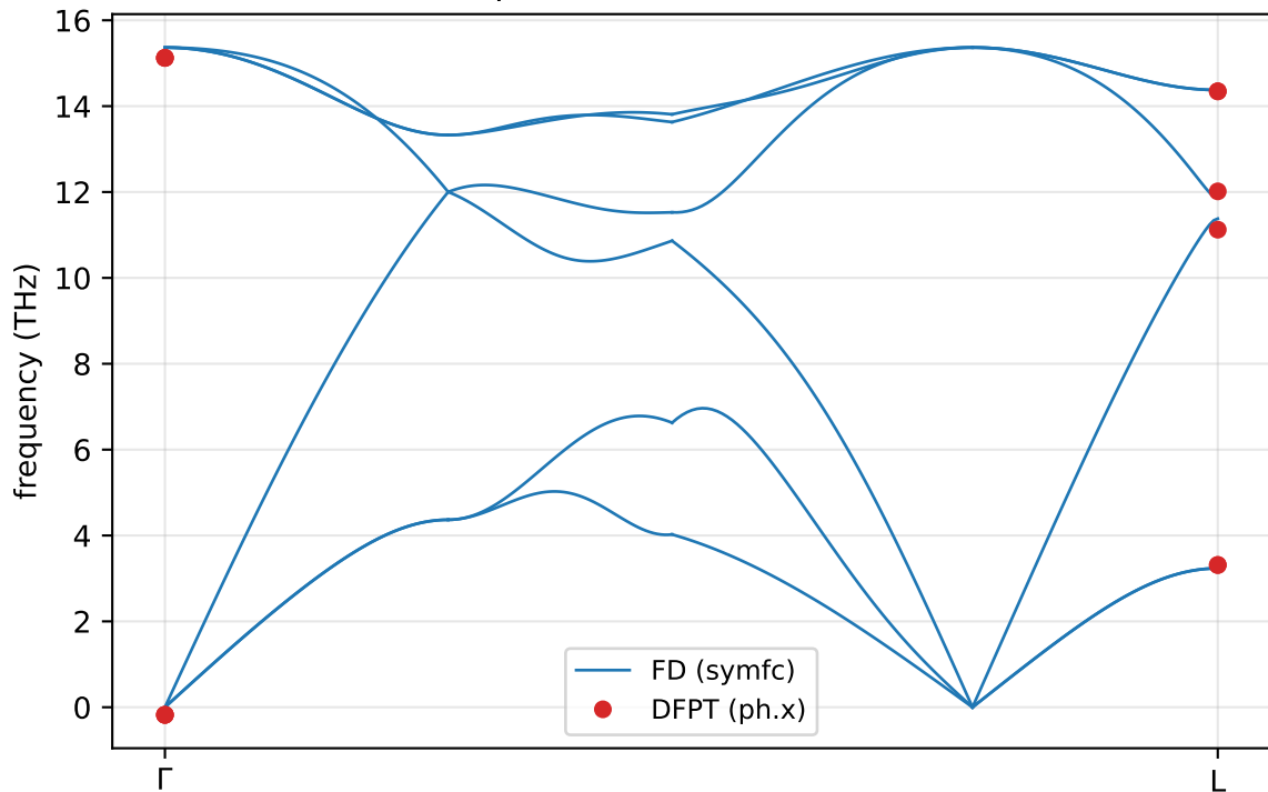
Bulk-Si dispersion: FD bands vs DFPT ( \Gamma , L)
