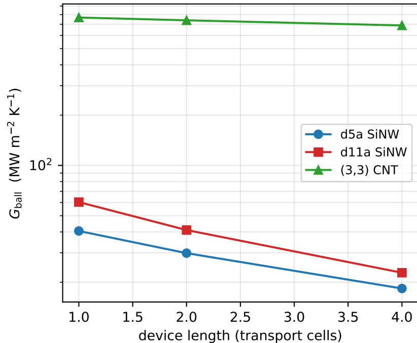
Ballistic conductance vs length (all wires)
