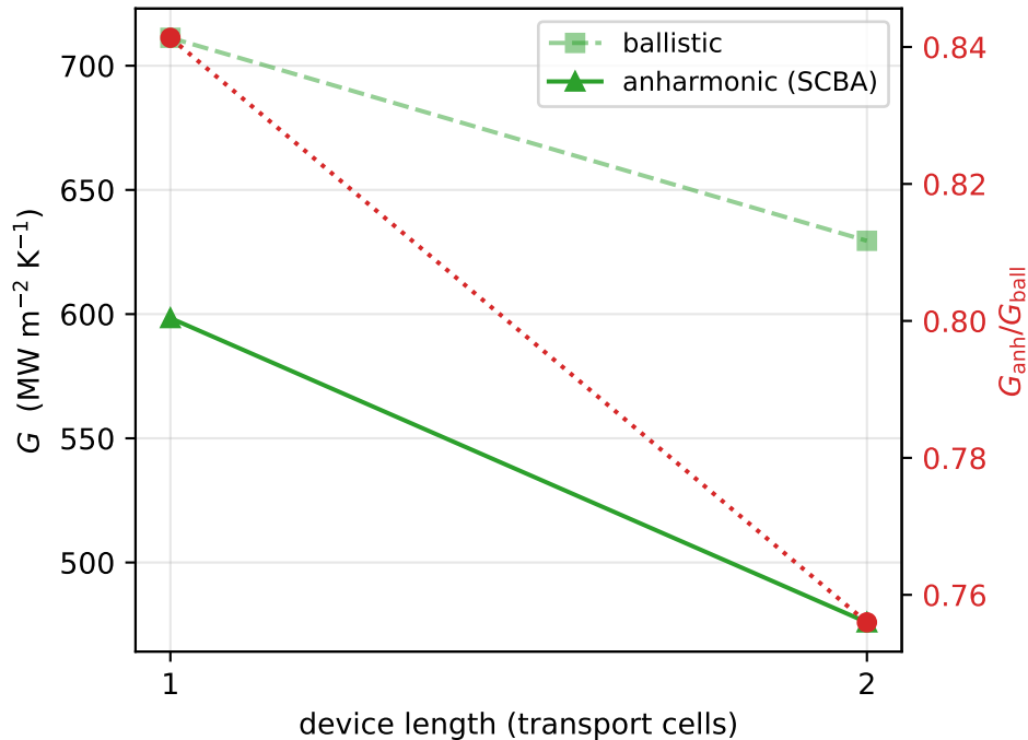
(3,3) CNT conductance vs length, T=300 K
