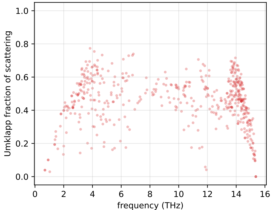
Normal vs Umklapp (Si 300 K, U=44%)
