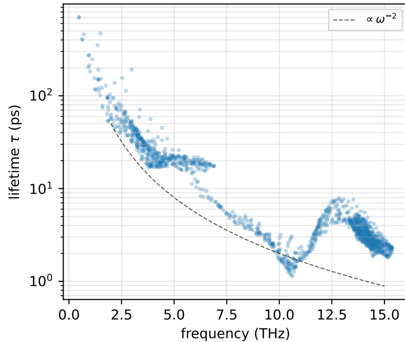
Phonon lifetimes, bulk Si 300 K
