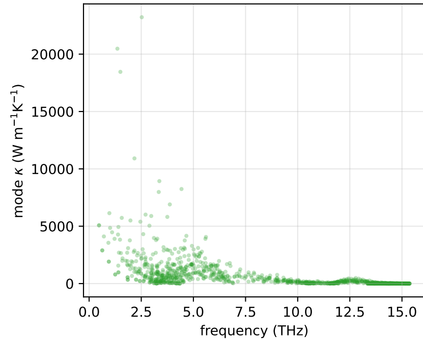
Mode-resolved \kappa spectrum
