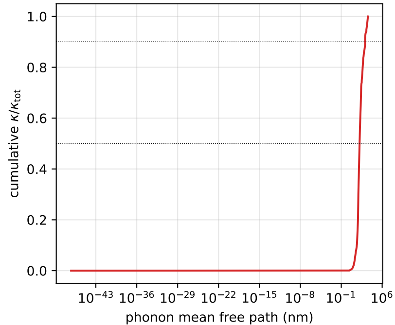
\kappa accumulation (50%@134nm, 90%@1216nm)
