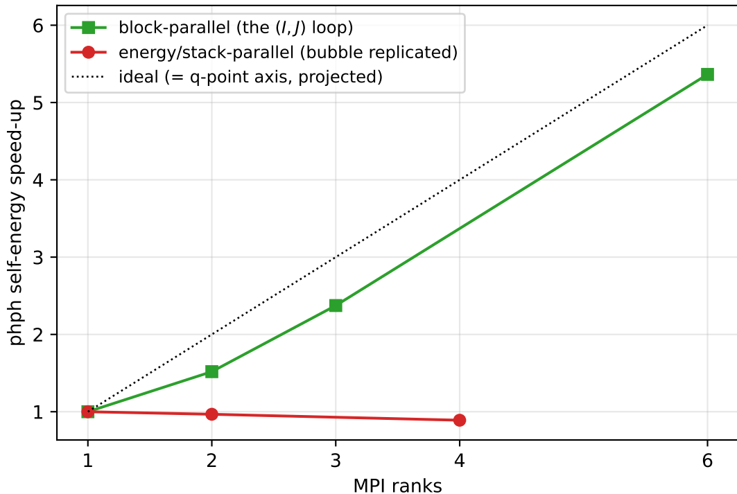
Distributed scaling of the quatrex 3-phonon self-energy
