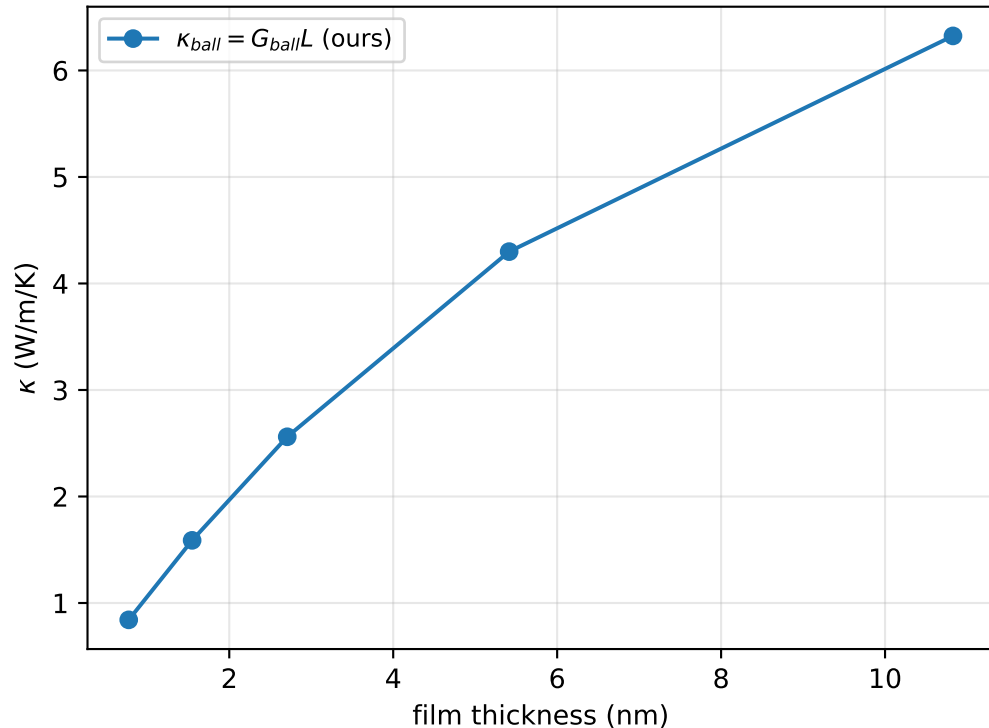
Ballistic \kappa rises \sim linearly in L
