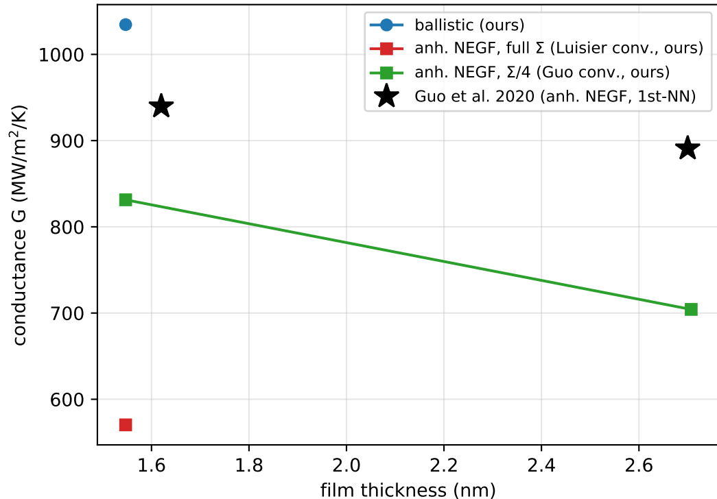
Cross-plane conductance vs thickness
